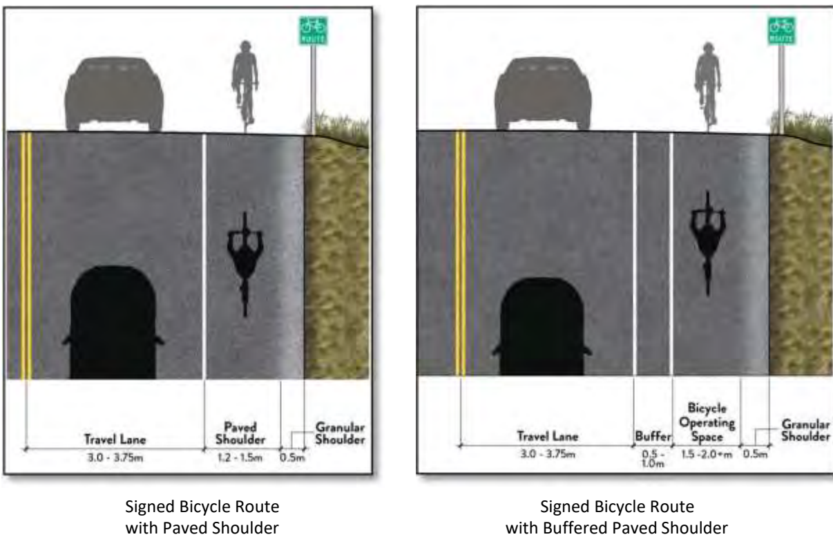
Figure C-10: Cross Sections and Plan Views of Paved Shoulders (Rural Cross-Sections)
