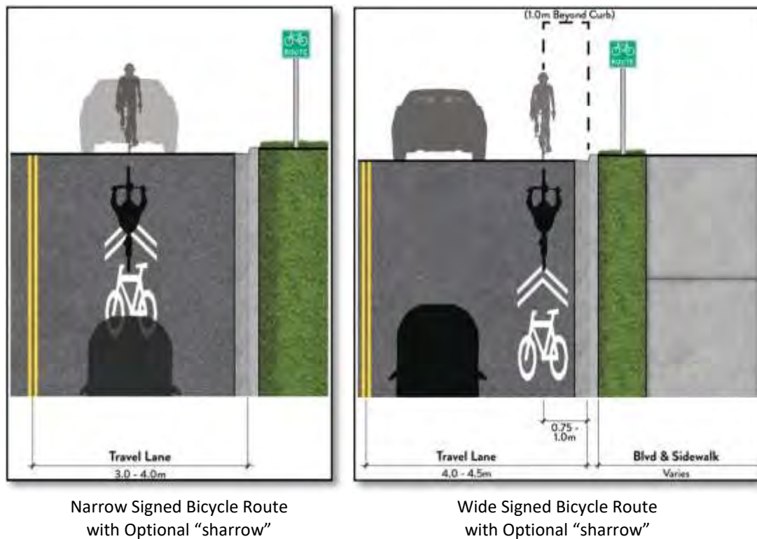
Figure C-9: Cross Sections and Plan Views of Shared Roadways and Signed Bicycle Routes
