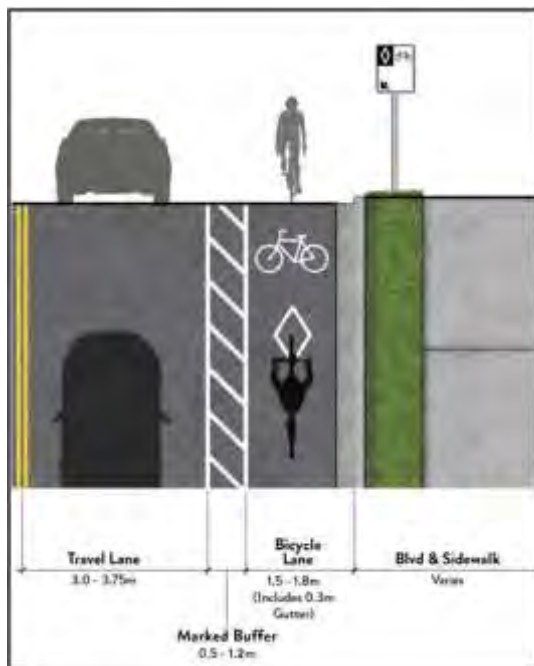
Buffered Bicycle Lane (Physical separation can be provided by including: flexible bollards, planters, or a concrete curb/median in the buffered area)
