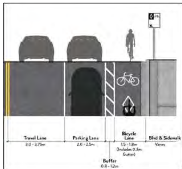
Parking Protected Bicycle Lane (Physical separation can be provided by including: flexible bollards, planters, or a concrete curb/median in the buffered area)
